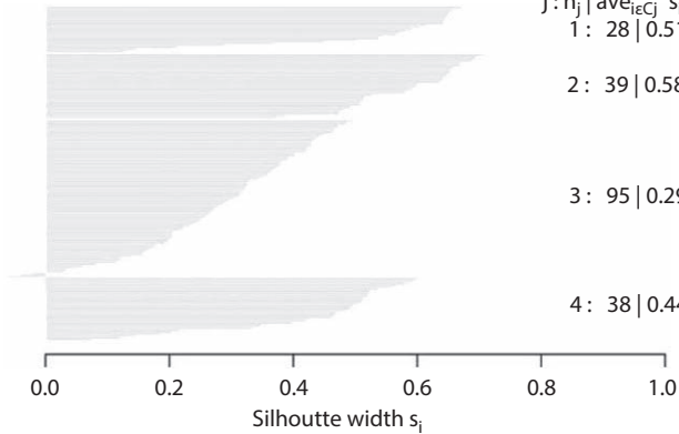
Silhouette plot of ( x = k4\$cluster , dist = dist(customer\_data[, 3:5] ,
