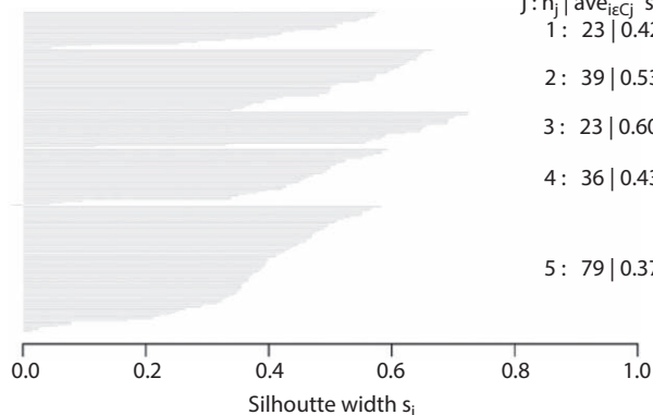
Silhouette plot of ( x = k5\$cluster , dist = dist(customer\_data[, 3:5] ,
